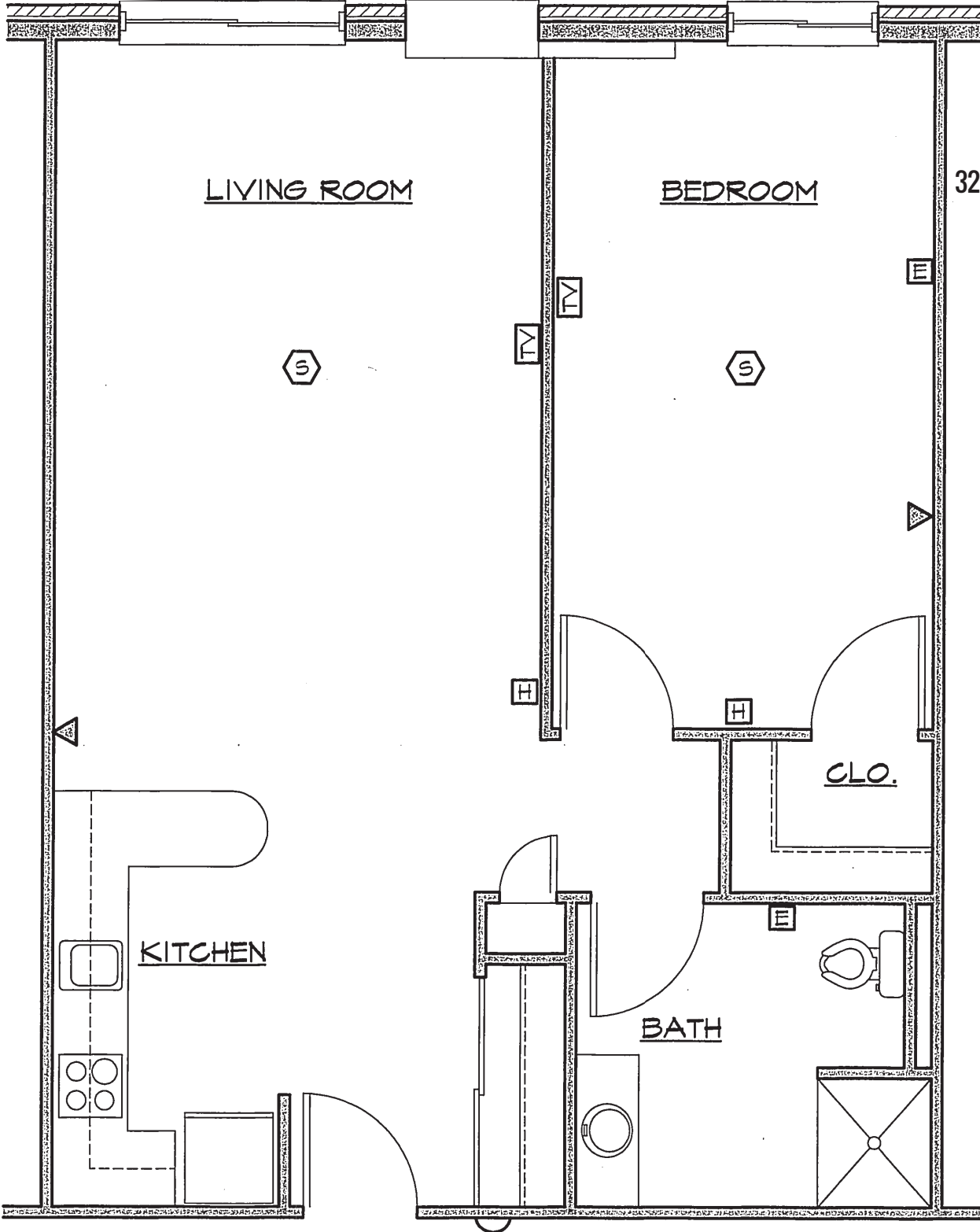
ENLARGED PLAN OF UNIT PLAN 'C' - ONE BEDROOM
